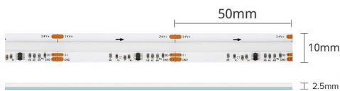
P20-COB, DC24V, 720Led/m, 5m, SPI RGB, 19W/m
