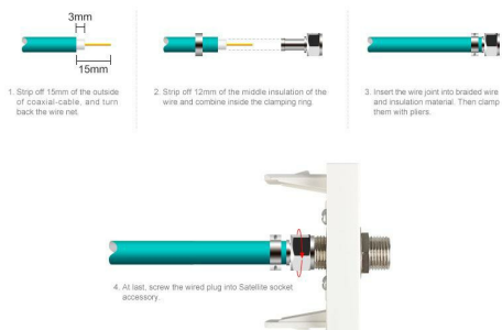
The wiring diagram of Satellite Socket
