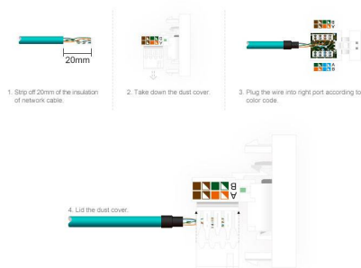
The wiring diagram of COM Socket
