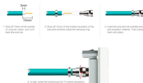
The wiring diagram of TV Socket
