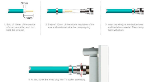
The wiring diagram of TV Socket
